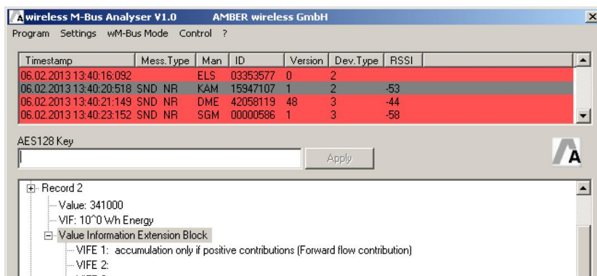
Figure 17: wM-Bus Frame Capture, Electricity Meter Decoded Record using wM-Bus Analyzer [73]
